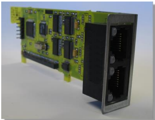
Single and dual RS-232 serial card with RJ-45 interface
