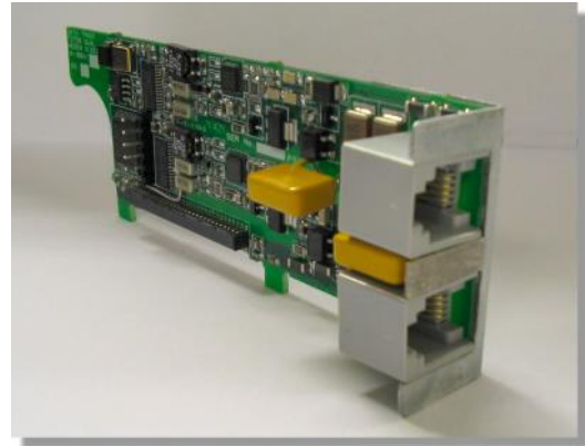
Single and dual V.92 PSTN modem card
